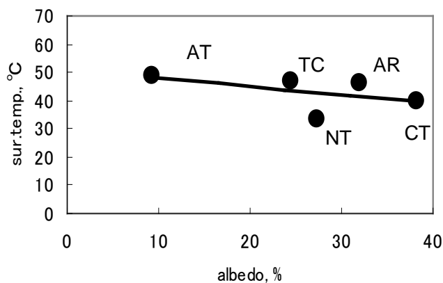
Fig. 1 Correlation between albedos and surface temperatures of outdoor sport surfaces (Aug.24,2006). AT: artificial turf, AR: artificial track, CT: clay track, NT: natural turf, TC: tennis court.
